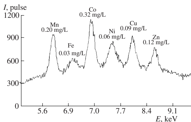
Fig. 2. X-ray fluorescence spectrum of a sorbent phase (KU-2X8) after the accumulation of trace components from a model solution in the presence of 0.25 g/L NaCl.
