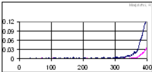
Fig. 2. The TL induced by X-ray irradiation in olivine from pallasites Brenham, Engle Station, Omolon and Marjalahti.
