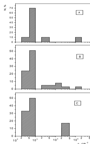
Fig. 1. Track-density distribution in the Brenham olivine crystals: A, B, C – different crystal.
