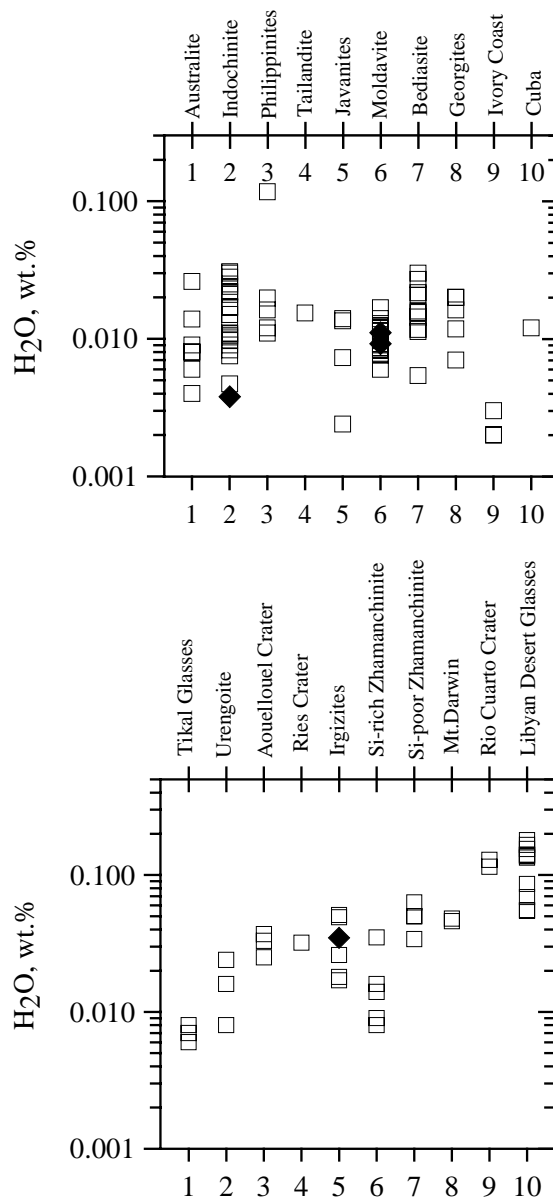
Fig.1. The water contents in various types of tektitic (top) and impactitic (bottom) glasses. Squares - available data from Gilchrist et al., 1969; King, Arndt, 1977; Frischat et al., 1982; Engelhardt et al., 1987; Koeberl, Beran, 1988; Newman et al., 1995; Beran, Koeberl, 1997. Diamonds - the data obtained in this investigation.
