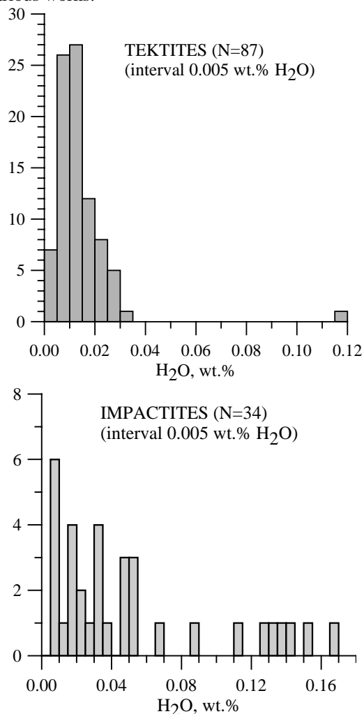
Fig.3. Histograms of H_2O concentrations in tektitic (top) and impactitic (bottom) glasses.
